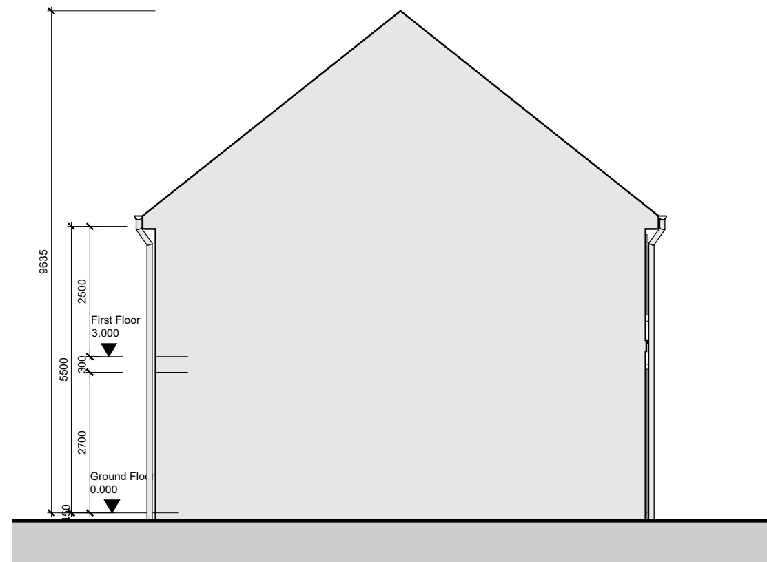
Side Elevation 01
